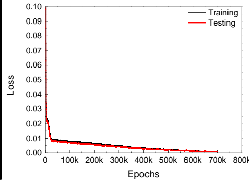
Training & Testing Loss Graph
