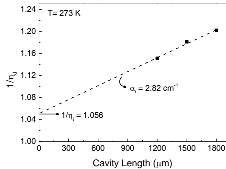
Internal loss validation
