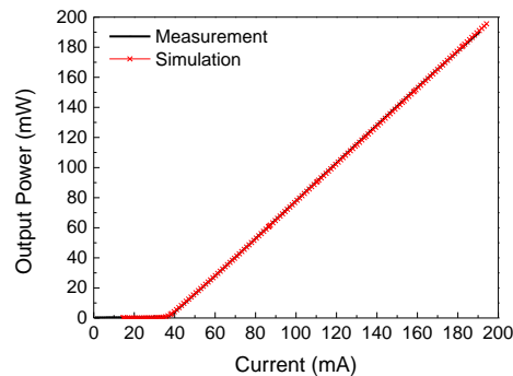
L-I characteristic validation
