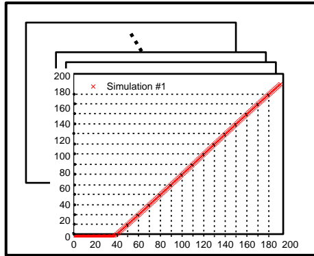
Training & Testing data input set
