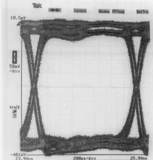
Fig. 8. Retimed data eyediagram from PRBS31
