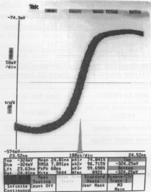
Fig. 7. Recovered clock jitter from PRBS31
