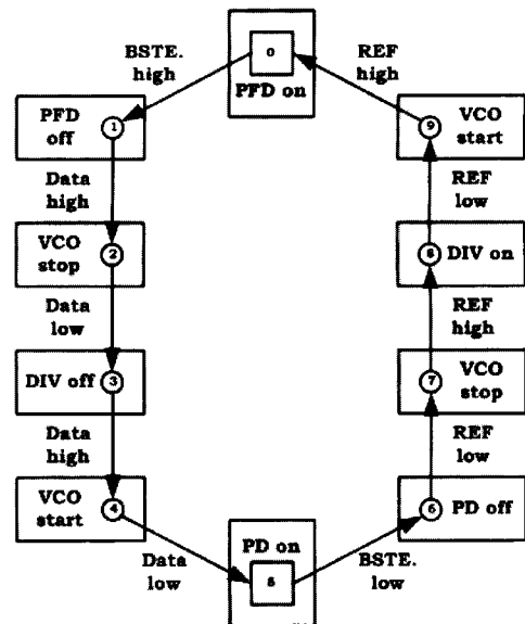
Fig. 4. Control circuit state diagram
