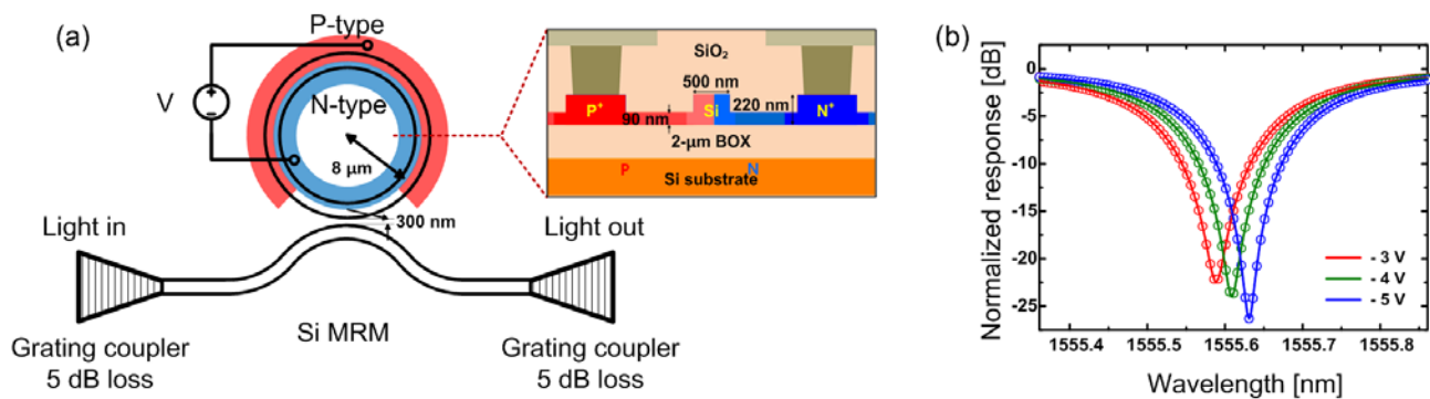
Fig. 1(a) Structure and cross section of Si MRM, (b) Measured and fitted normalized transmission characteristics.
