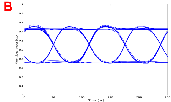
<Transient simulation – extracting eye diagram>
