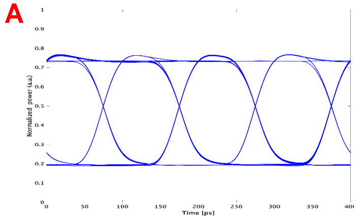
<Transient simulation – extracting eye diagram>
