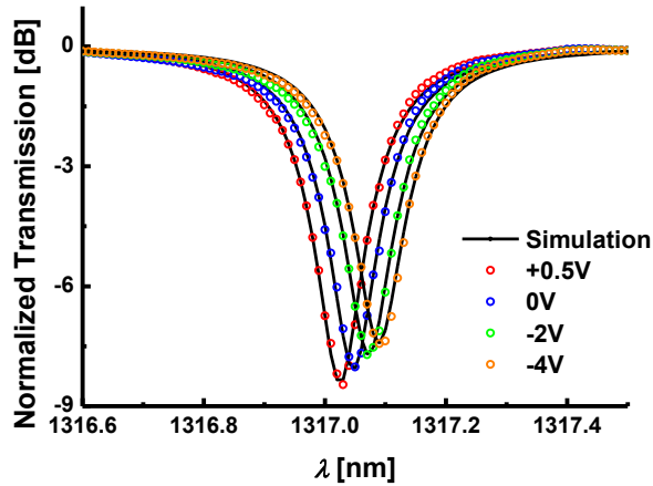
<Measured Transmission Curve>
